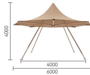
Dimension Drawing
