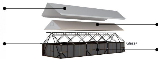
T9Exploded View
