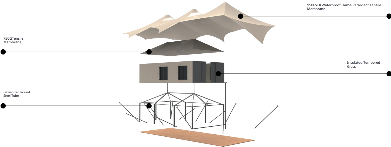
ShanluanExploded View
