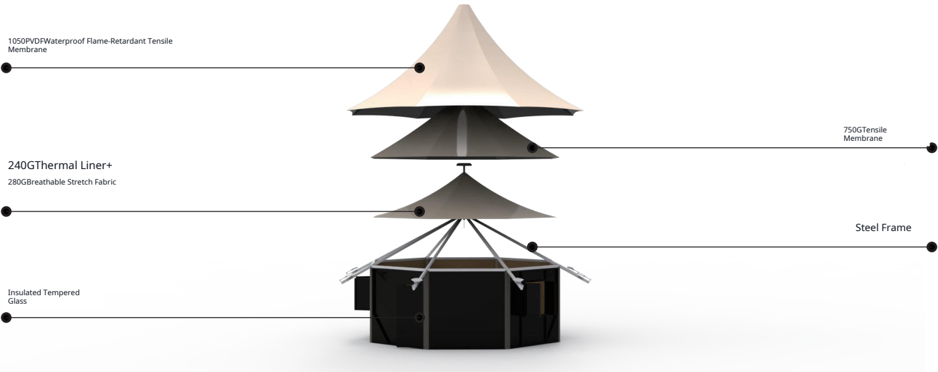
Octagonal Glass TentExploded View
