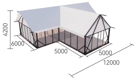
TDimension Drawing
