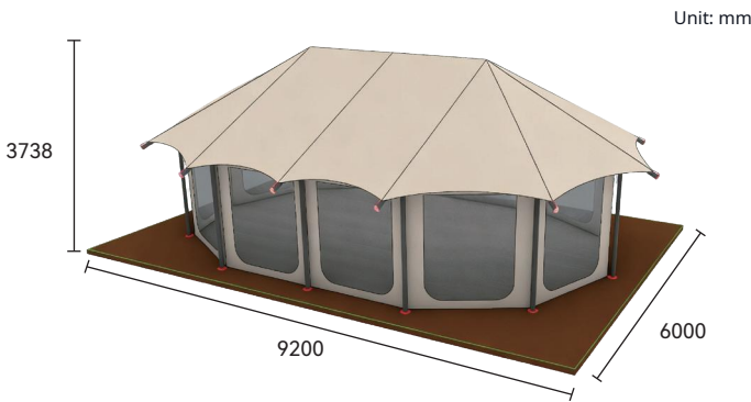
YunluDimension Drawing
