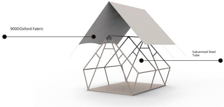
Exploded View
