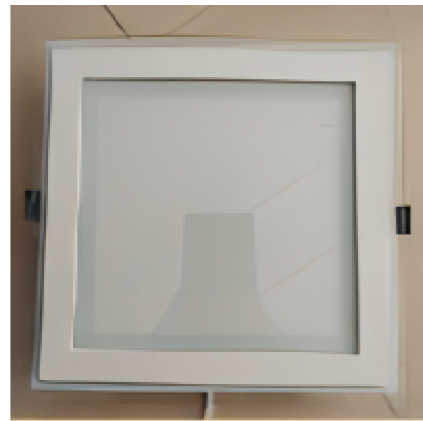
206F/18W MAT: ABS+GLASS SIZE: 180*180MM CUTOUT SIZE: 140*140MM 3000K/4000K/6500K
