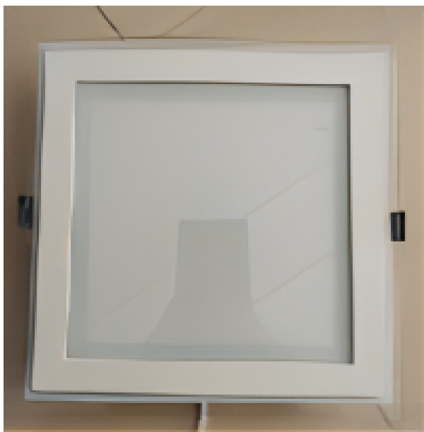
206F/12W MAT: ABS+GLASS SIZE: 150*150MM CUTOUT SIZE: 110*110MM 3000K/4000K/6500K
